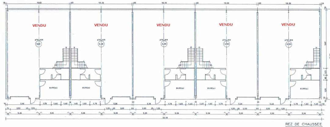
Plans RDC - ETAGE
